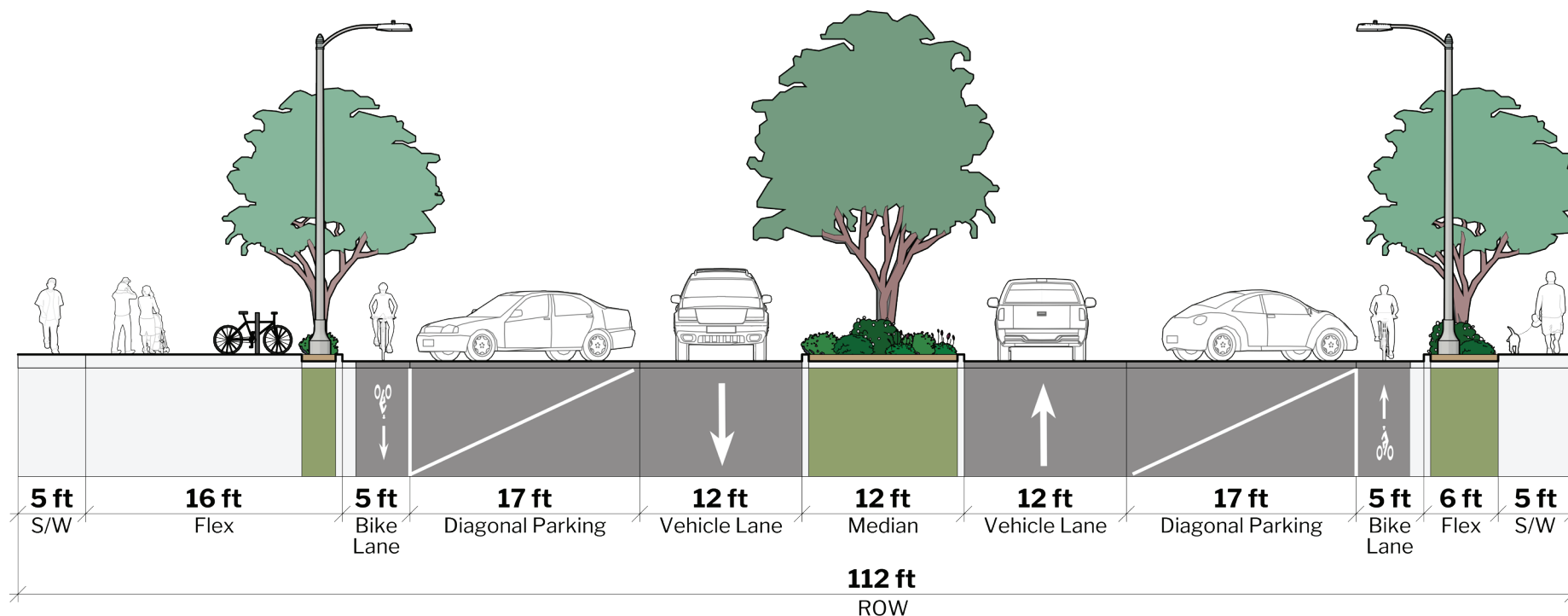
FIGURE 7-3: Village Promenade Special Treatment Area Cross Section
