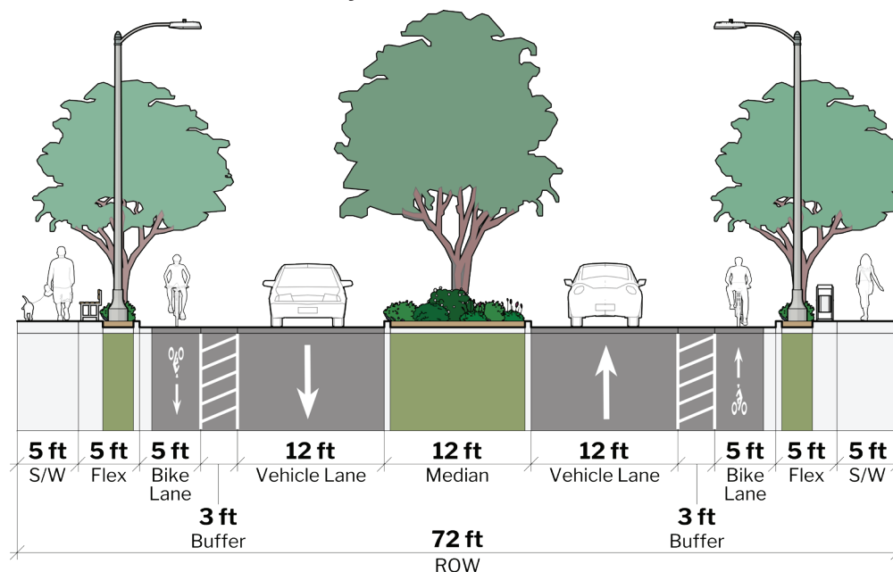
FIGURE 7-8: Class II Collector Bicycle Cross Section
