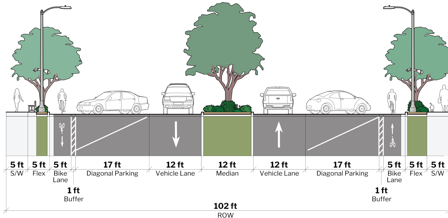
FIGURE 7-4: East Broadway Special Treatment Area Cross Section
