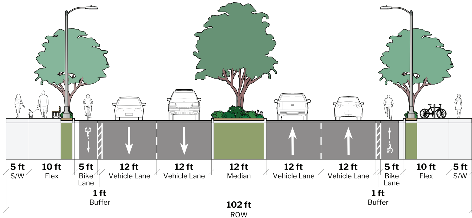
FIGURE 7-5: Mixed-Use Promenade Special Treatment Area Cross Section
