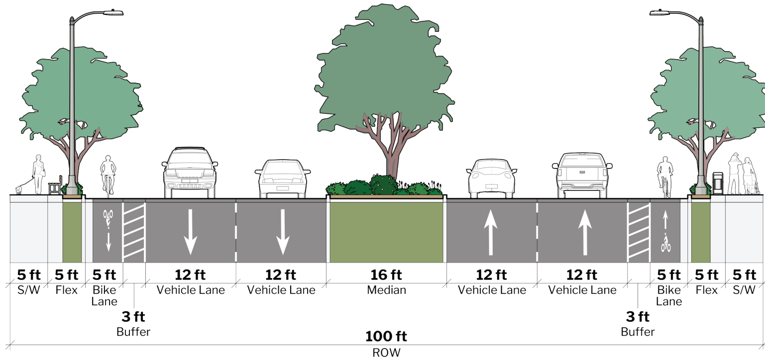
FIGURE 7-6: Class I Collector Cross Section
