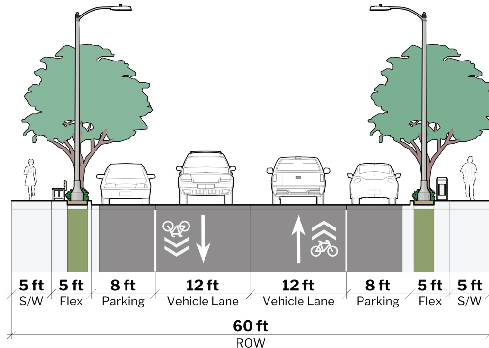
FIGURE 7-9: Class III Collector Bicycle Cross Section
