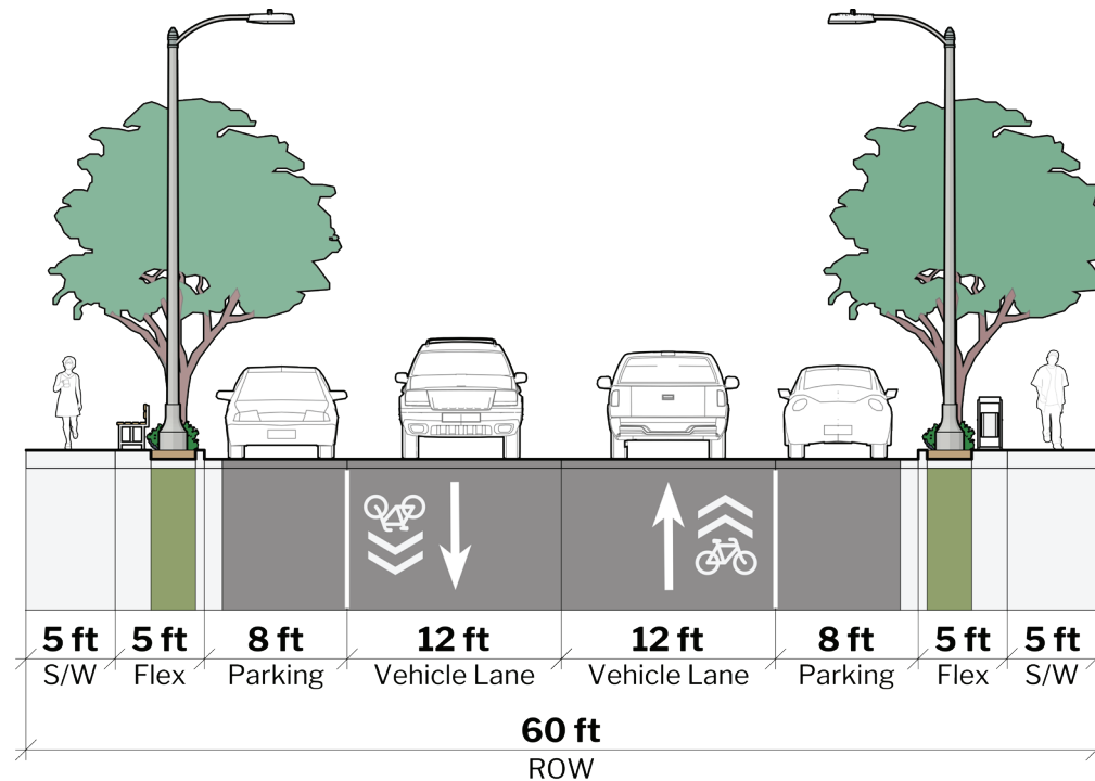
FIGURE 7-10: Neighborhood Street Cross Section
