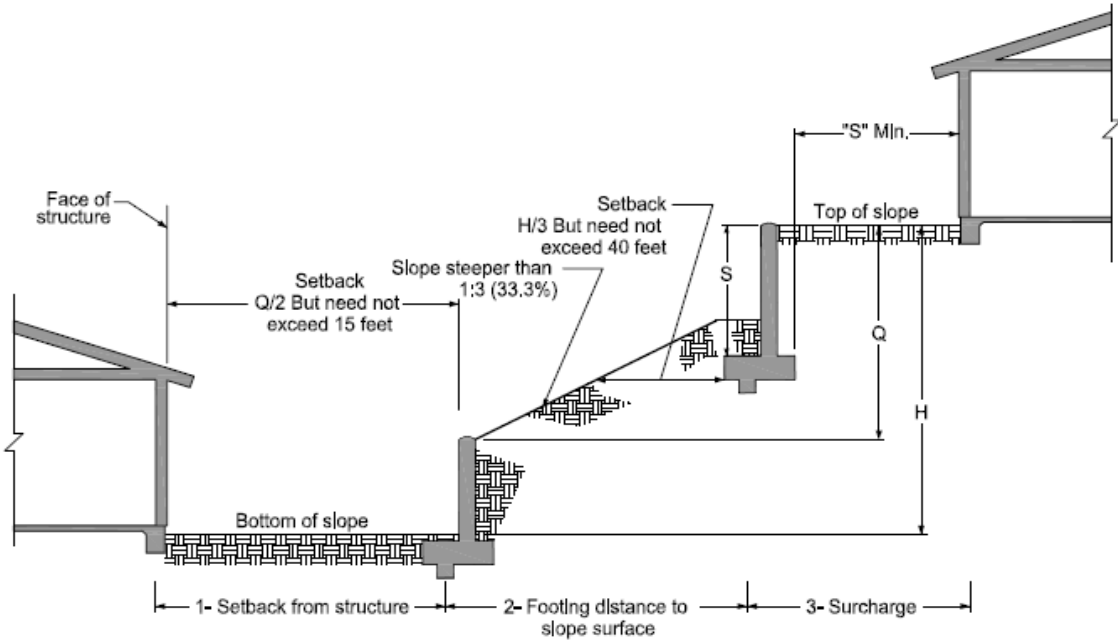
Figure 1 / Subcharge and Slope Setbacks
